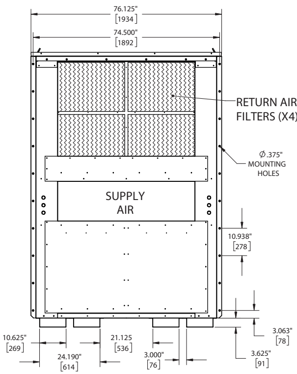
REAR VIEW
