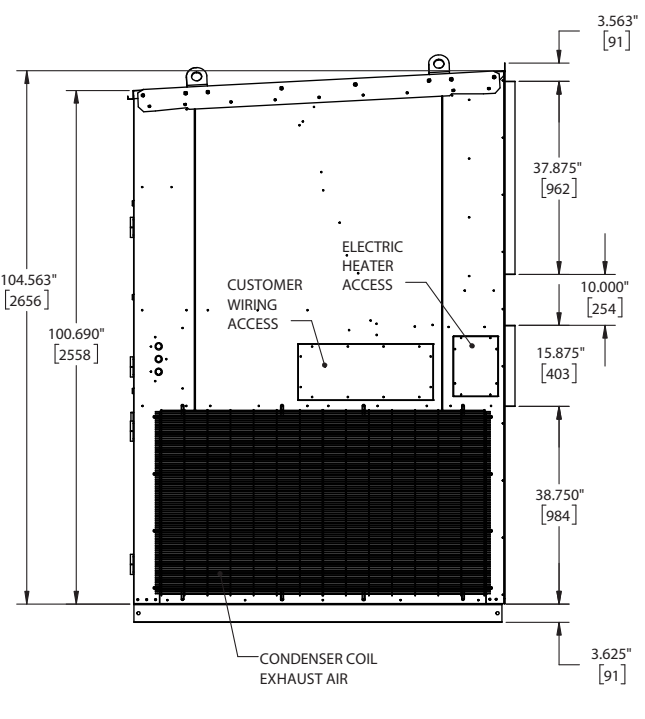
RIGHT VIEW
