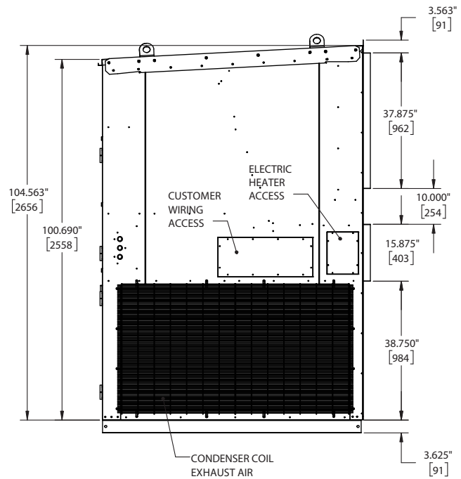
RIGHT VIEW
