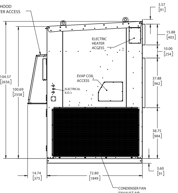
RIGHT VIEW
