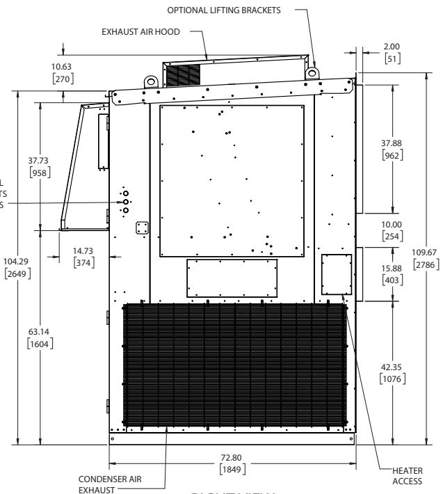
RIGHT VIEW
