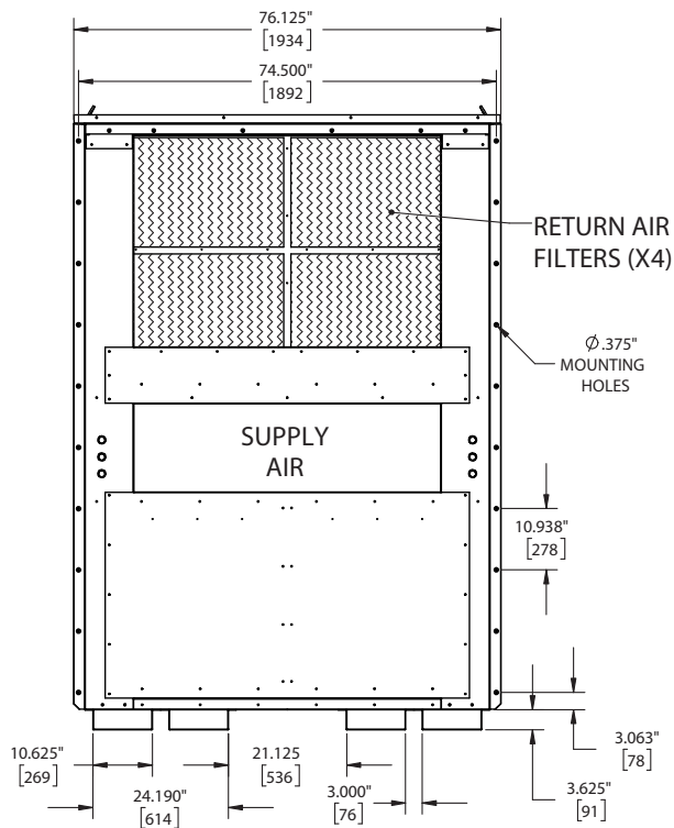
REAR VIEW
